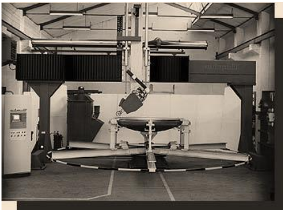
CNC installations for stainless steel tank ends and bodies, up to 8-meter diameter.
