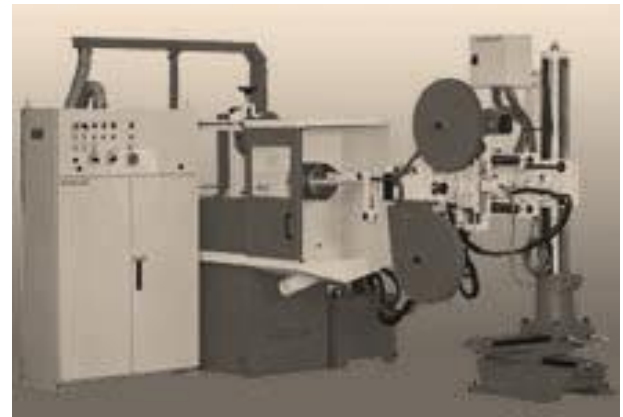
Machine with a single spindle Model IRM/1UT for grinding and satin finishing of round parts (in & out).
